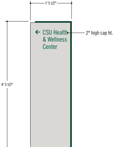
XX - PEDESTRIAN DIRECTIONAL FRONT ELEVATION SCALE: 3/4"=1'
