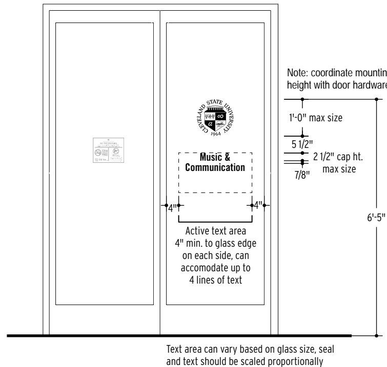
TYPICAL ELEVATION (CONDITIONS WILL VARY) SCALE: 3/8" = 1'
