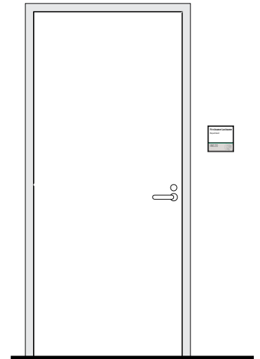
Typical Room ID Mounting (G4)
