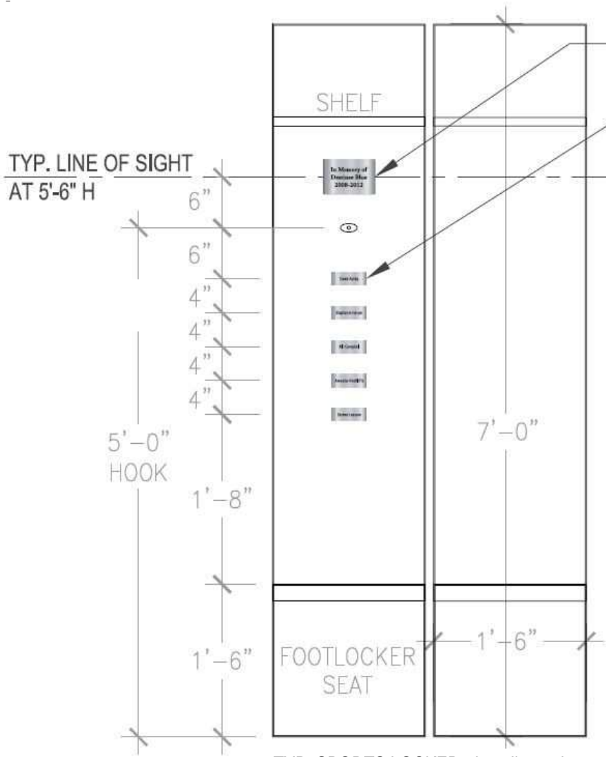
TYP. SPORTS LOCKER - install template
