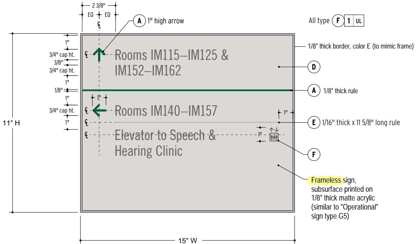
DETAIL - LARGE = 6-8 LINES OF TEXT SCALE: 3" = 1'
