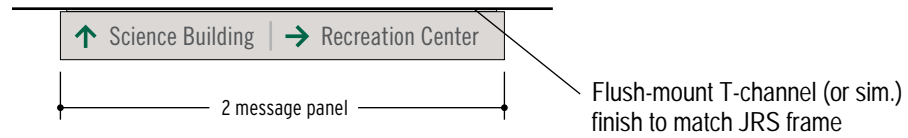
ELEVATION (ALT : (2) MESSAGES) SCALE: 3/8" = 1'
